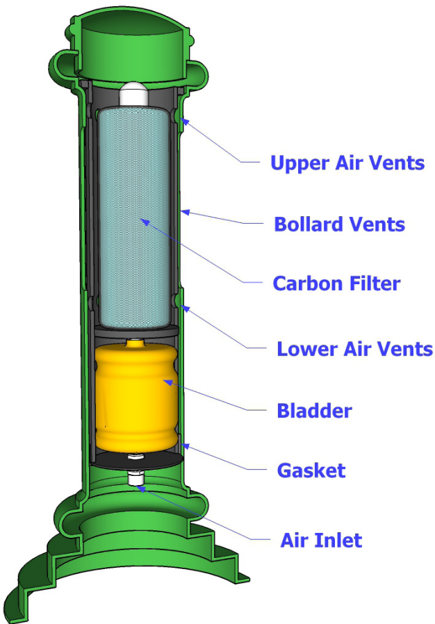
Typical gas and air flow through bollard vent or manhole cover.
