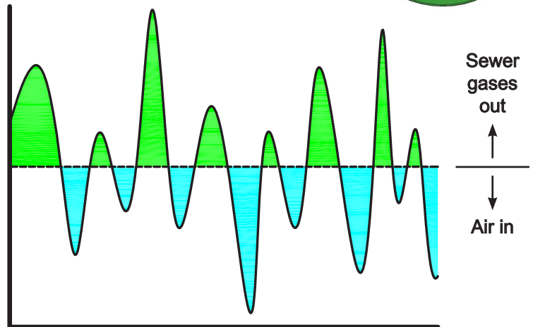
Typical gas and air flow through bollard vent or manhole cover.
