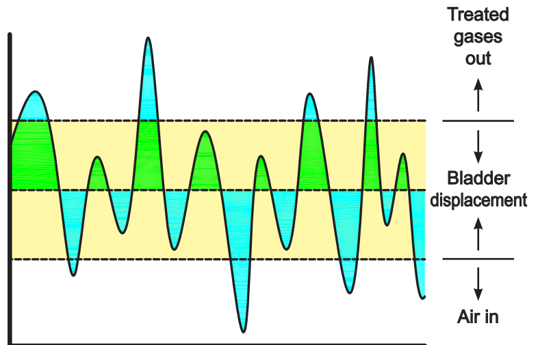
Only sewer gases that exceed bladder capacity need to be treated. This greatly extends carbon life.
