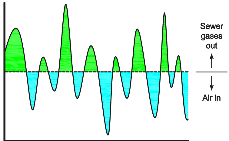
Typical gas and air flow through manhole cover.
